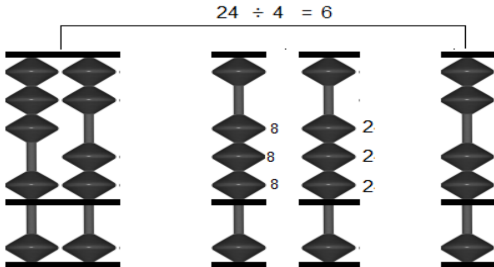
Fig. 1. Division Demonstration Using the Libyan-American Abacus
